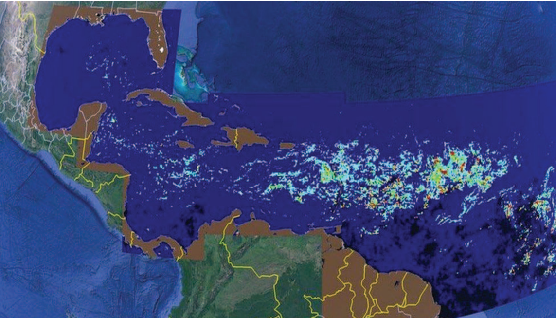
IMAGE SOURCE,UNIVERSITY OF SOUTH FLORIDA OPTICAL OCEANOGRAPHY Satellite imaging shows the scale of the seaweed belt
